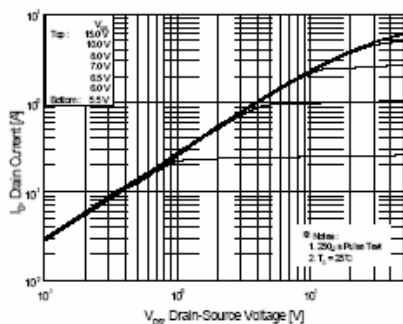
Figure 1. On-Region Characteristics
