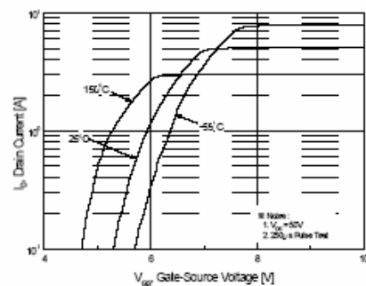
Figure 2. Transfer Characteristics
