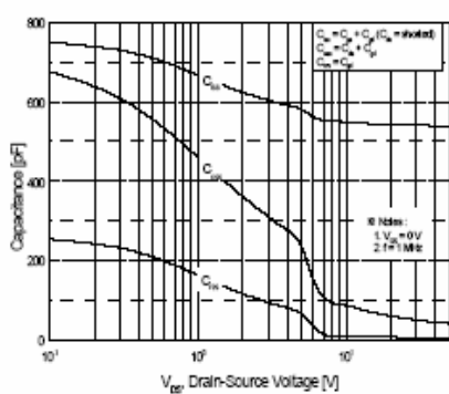
Figure 5. Capacitance Characteristics
