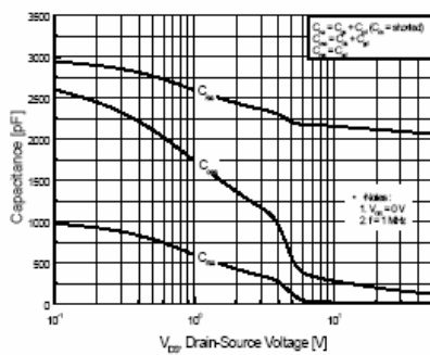
Figure 5. Capacitance Characteristics
