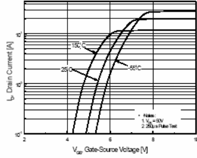
Figure 2. Transfer Characteristics
