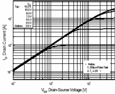
Figure 1. On-Region Characteristics
