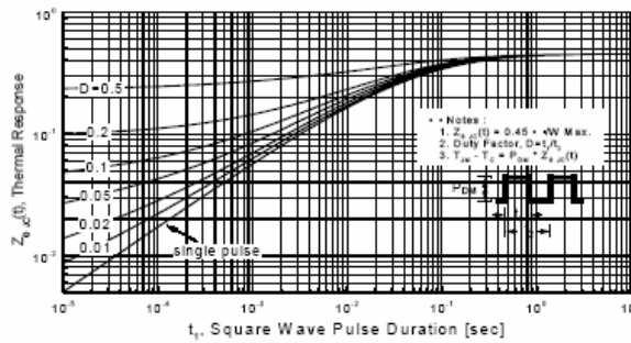
Figure 11. Transient Thermal Response Curve
