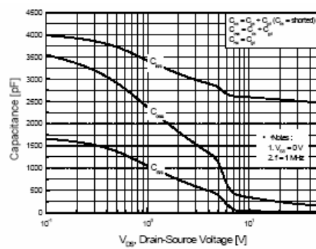
Figure 5. Capacitance Characteristics
