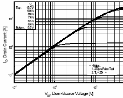
Figure 1. On-Region Characteristics
