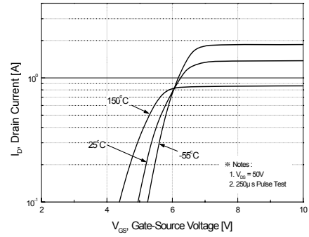
Figure 2. Transfer Characteristics
