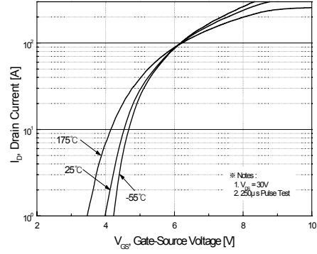
Figure 2. Transfer Characteristics
