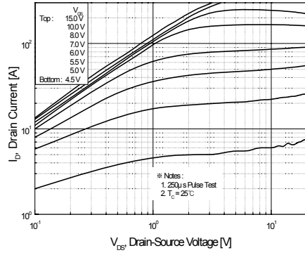
Figure 1. On-Region Characteristics
