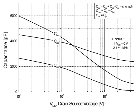
Figure 5. Capacitance Characteristics
