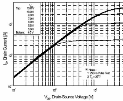
Figure 1. On-Region Characteristics
