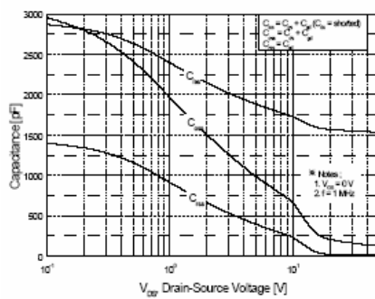
Figure 5. Capacitance Characteristics
