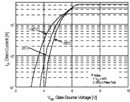
Figure 2. Transfer Characteristics
