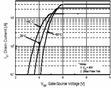
Figure 2. Transfer Characteristics
